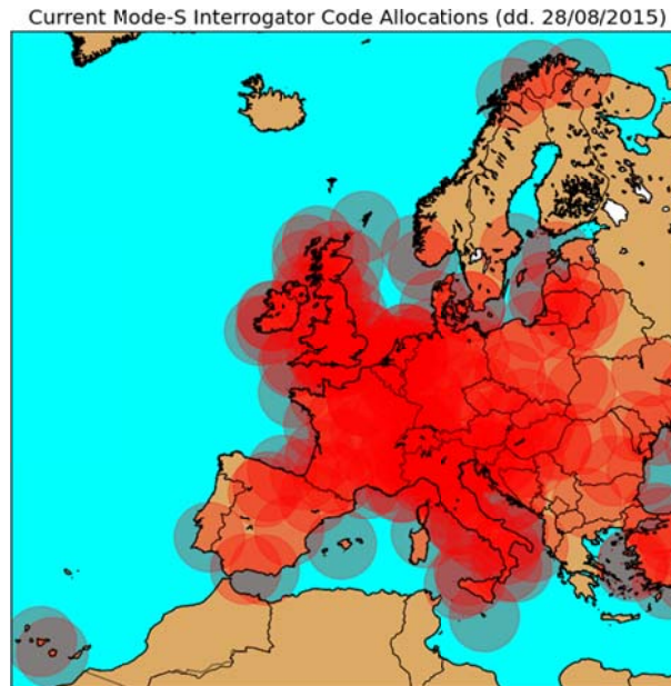
Figure 16 : Coverage of Mode-S ELS or EHS (see Figure 5 and Figure 6) radars 8 in Europe using a default radius of 200km. As Mode-S ELS and EHS use the same ground infrastructure, this graph shows the enormous future potential for EHS interrogation by ATC. However, updating from ELS to EHS is not trivial for air traffic organizations and results, amongst others, in a significant increase of data load on ATC networks.
