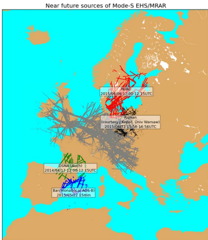
Figure 15 : The coverage of known Mode-S EHS/MRAR information. Some locations are in test phase like in Auch (France) and Denmark and is expected to become operational in the near future, and is to be extended as shown in the previous figure on EU regulations.
